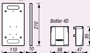
Platine support
